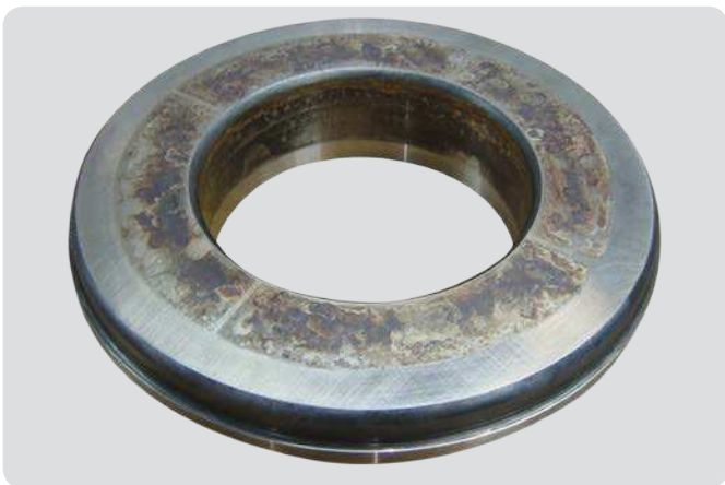
Spherical roller thrust bearing shaft washer Inadequate seat
