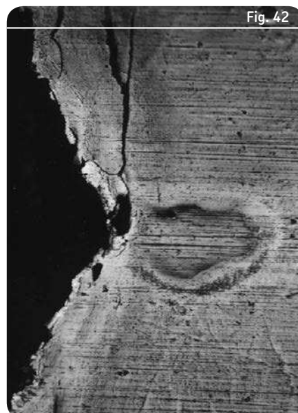
Spalling resulting from an indentation in a spherical roller bearing
