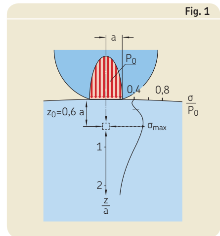
Fig. 1 Compressive and shear stresses beneath the raceway
