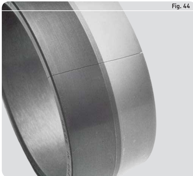
Fractured inner ring of a spherical roller bearing with a tapered bore resulting from excessive drive-up
